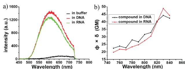
Fig. 2 a: Two-photon excited fluorescence spectra of 2,7-9E-BHVC in the absence and in the presence of DNA or RNA with 100 : 1 [NA]/[dyes] ratio. b: Two-photon action absorption spectra of 2,7-9E-BHVC in DNA and RNA with 100 : 1 [NA]/[dyes] ratio. Compound concentration: 1.0 \times 10^{-5} M.
